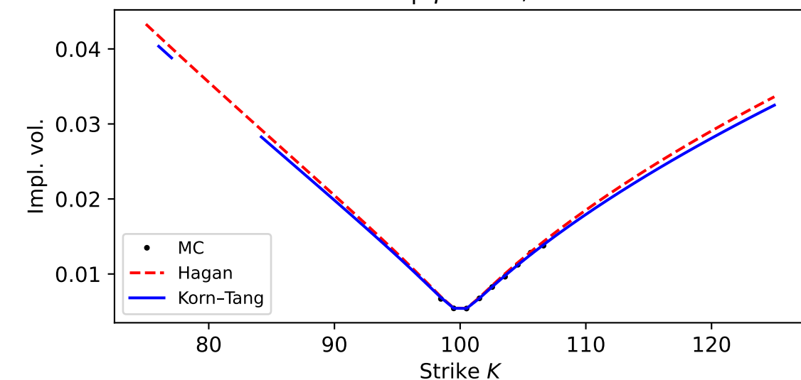
IV smile | \rho = -0.7, \nu = 0.9
