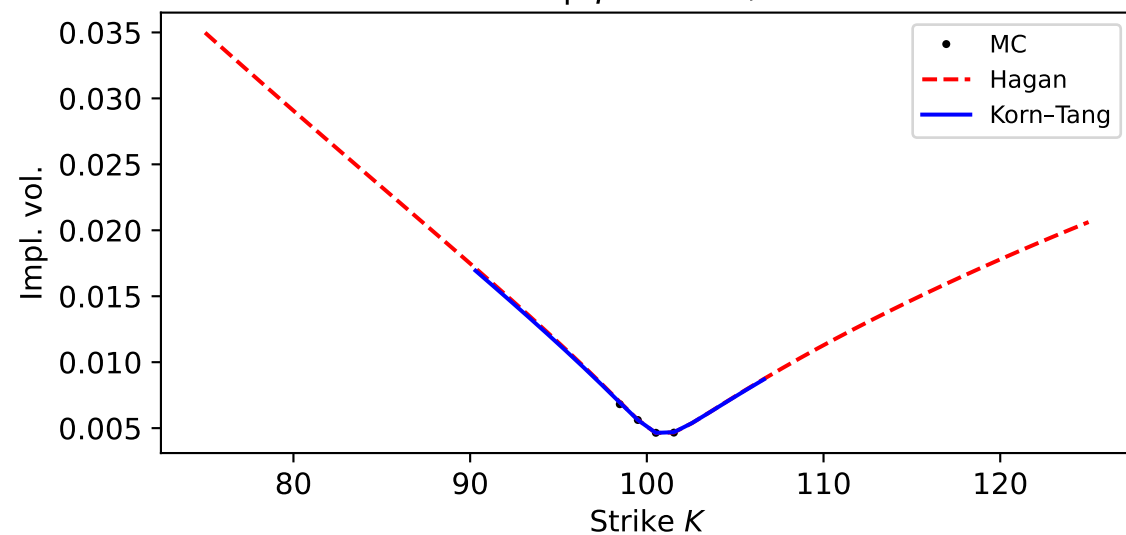
IV smile | \rho = 0.0, \nu = 0.6
