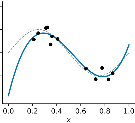
degree 3 train MSE = 0.043
