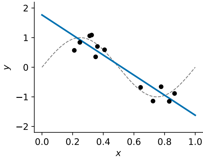
degree 1 train MSE = 0.089
