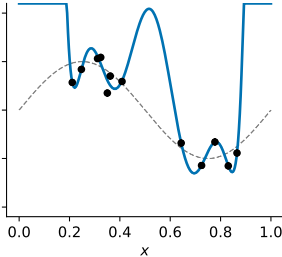
degree 9 train MSE = 0.011
