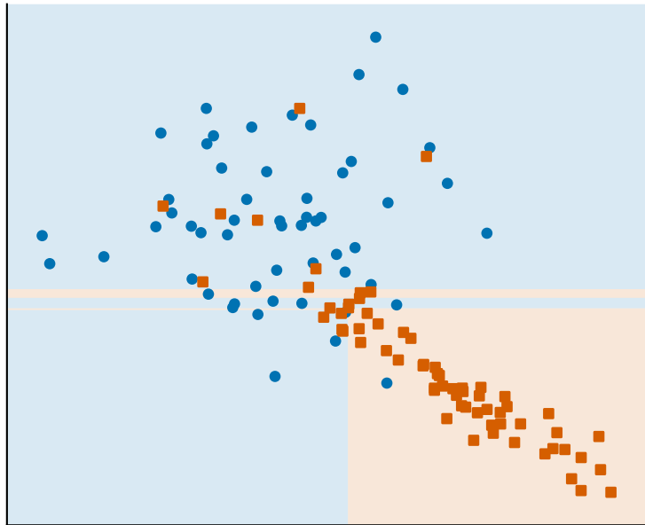
bootstrap 2: root split x_2 \leq -0.03
