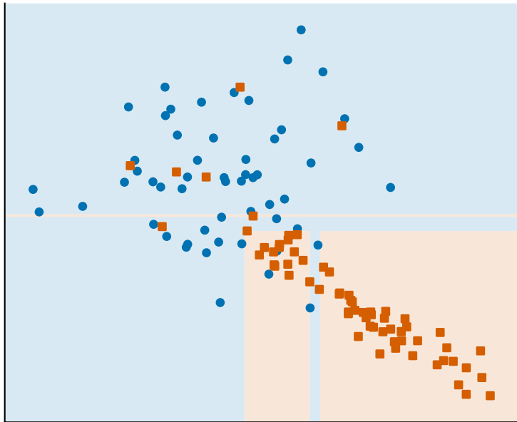
bootstrap 1: root split x_2 \leq 0.22
