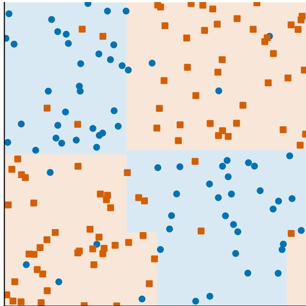
tree, depth 3 train acc = 0.89
