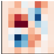
k = 16
