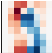
k = 8
