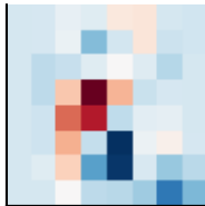
k = 64
