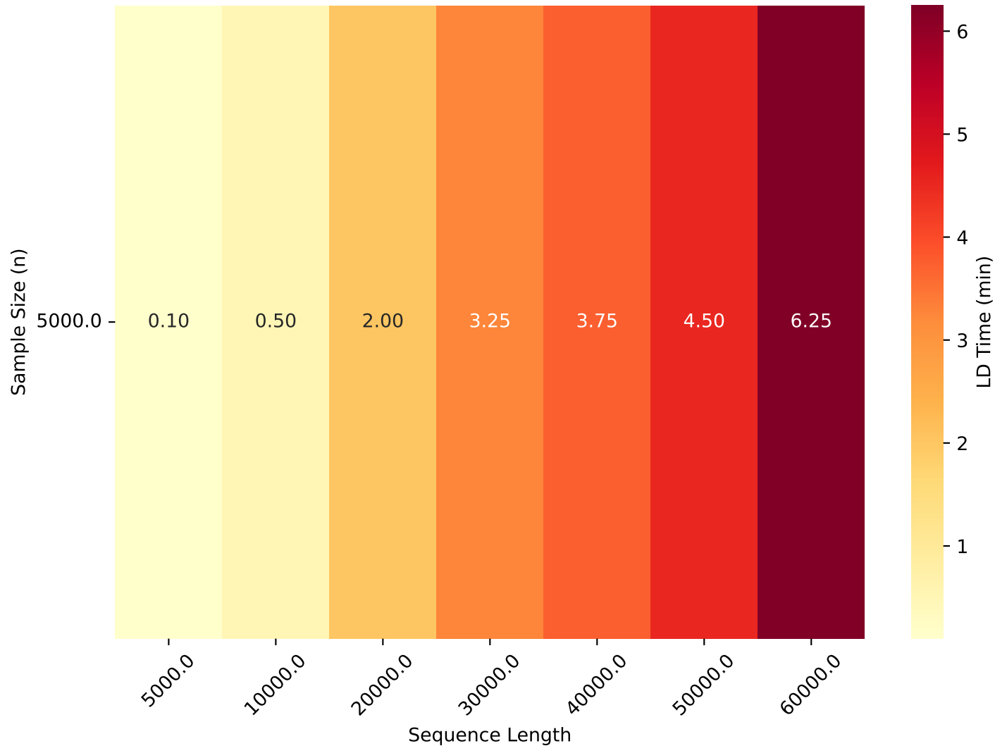
LD Time Heatmap (LD Window = 100)
