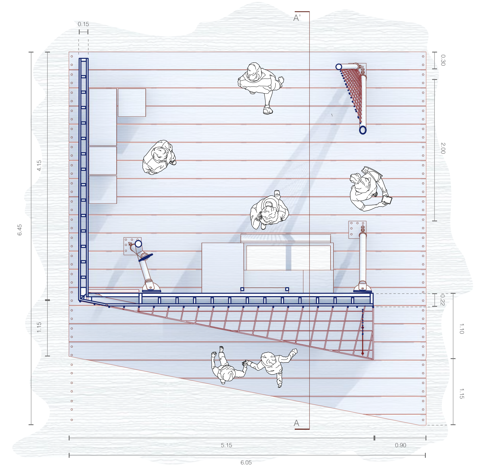
Floor plan
