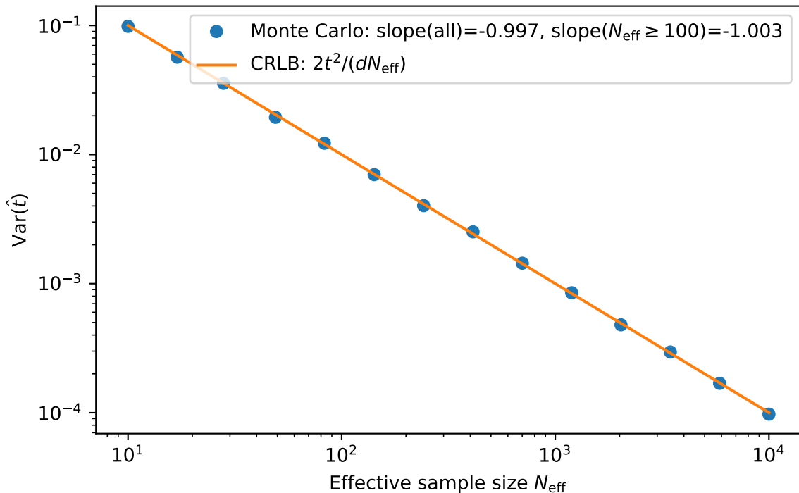
CRLB verification for time estimation (normal diffusion)
