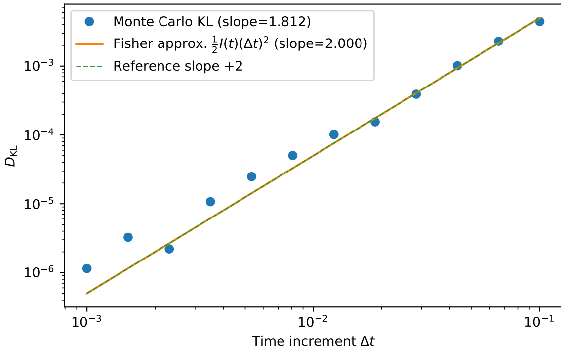
KL divergence vs Fisher information (local regime)
