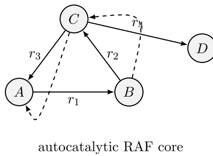
Рис. 16: RAF network as a chemical continuum at level K_3 .
