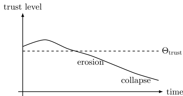
Рис. 27: Trust thresholds and collapse of social continuumness.
