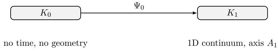
Рис. 8: Schematic of the transition \Psi_{0 \rightarrow 1} from the substrate K_0 to the first continuum K_1 .
