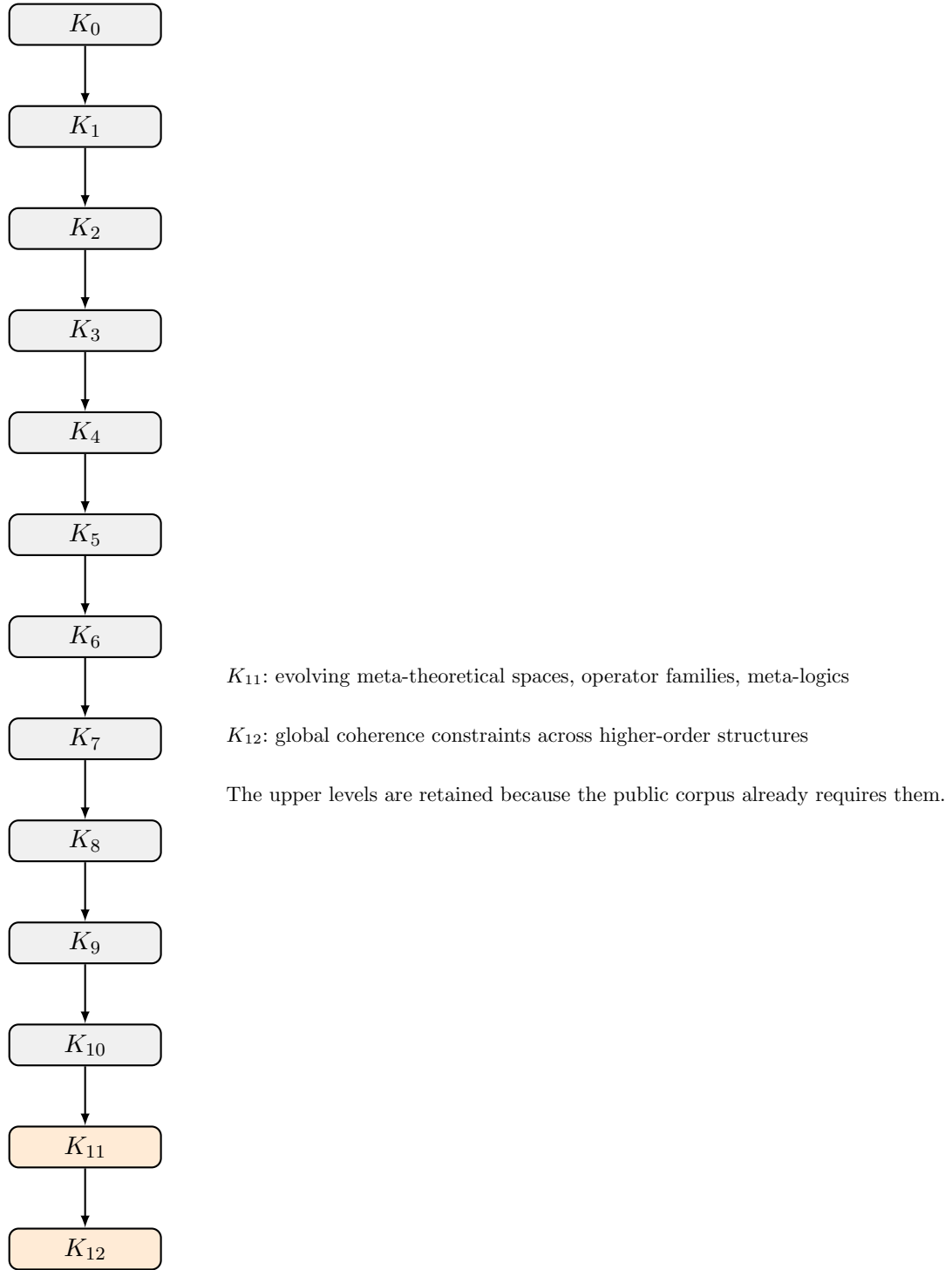
Рис. 3: Extended vertical hierarchy through K_{12} . The added upper levels are justified by the need to represent evolving meta-theoretical spaces and their global coherence conditions rather than by decorative level inflation.
