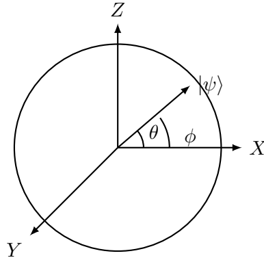
Рис. 15: Illustrative Bloch sphere diagram for quantum two-level systems.
