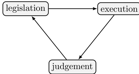
C_7 : institutional cycle
