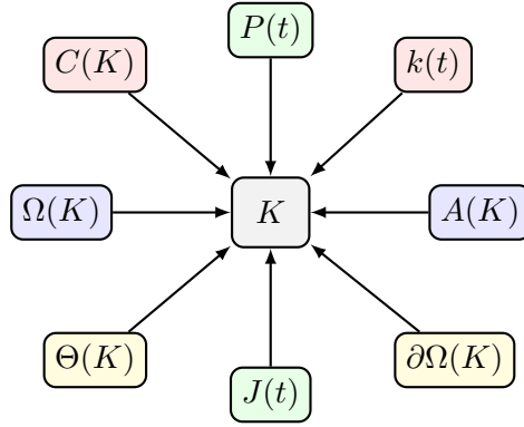
Рис. 4: Schematic structure of a continuum K = (\Omega, A, P, J, \Theta, \partial\Omega, C, k) .
