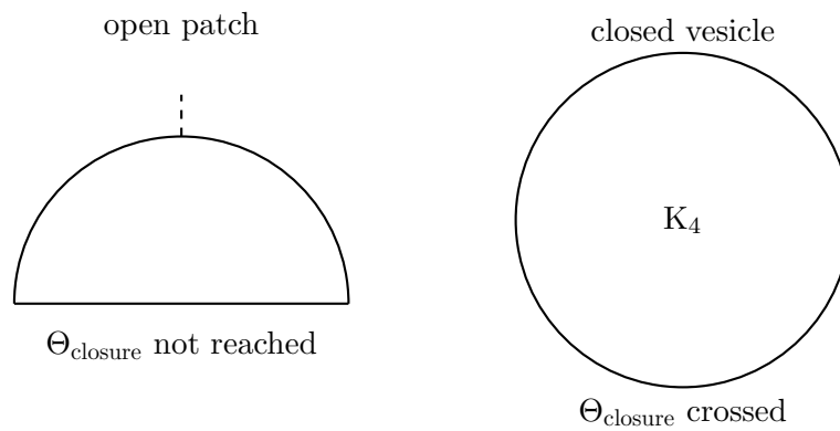
Рис. 18: Membrane closure and emergence of a protocellular boundary at level K_4 .
