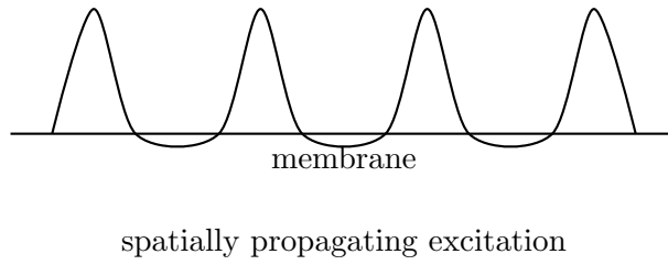
Рис. 21: Propagation of membrane potential \Delta V along a boundary.
