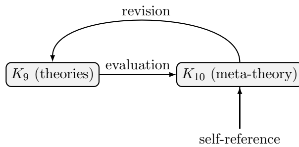
Рис. 32: Self-referential structure of meta-theoretical continua at level K_{10} .
