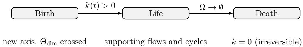
Рис. 2: Minimal life-cycle schematic for the bounded collapse grammar. The point of the figure is not to offer a domain-specific simulation but to show the exact interpretive burden of the formal rules: positive continuumness keeps the object live; admissible-state collapse kills it; any later continuation must be classified under rebirth rather than persistence.
