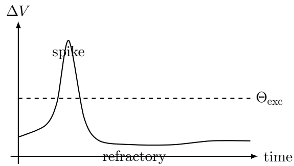
Рис. 23: Proto-spike dynamics as a minimal excitatory cycle.
