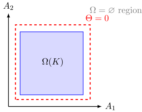
Рис. 5: Axes and threshold surfaces in the extended state space of a continuum.
