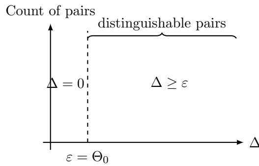
Рис. 7: Structural difference and minimal threshold \Theta_0 at level K_0 .
