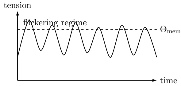
Рис. 20: Vesicle flickering regime near curvature and osmotic thresholds.
