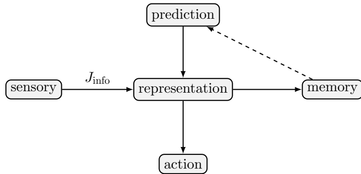
Рис. 31: Flows between representations, models and data in K_9 .
