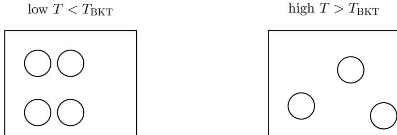
Рис. 14: BKT-type transition as an example of threshold-governed emergence of a new topological axis.
