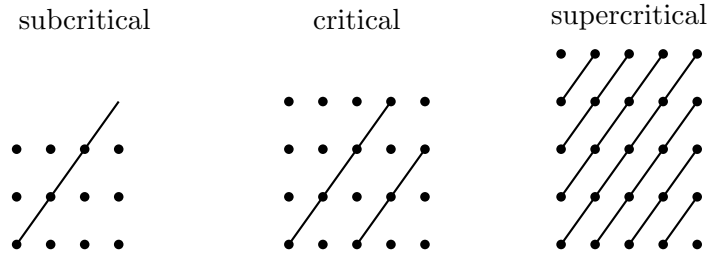
Рис. 13: Percolation-type transition at level K_2 .
