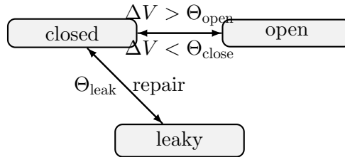
Рис. 22: Ion channel states and excitation thresholds at level K_5 .
