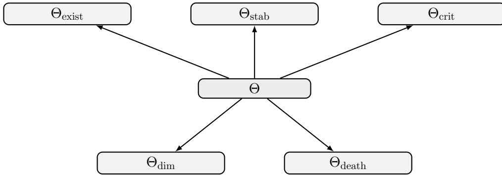
Рис. 6: Taxonomy of thresholds: existence, stability, critical, dimensional and death thresholds.
