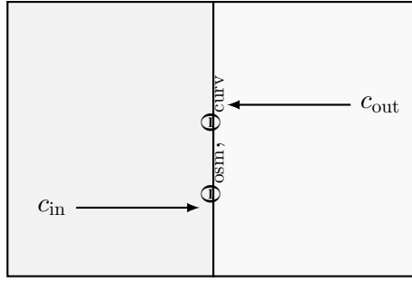
Рис. 19: Osmotic gradients, membrane tension and structural thresholds in protocells.
