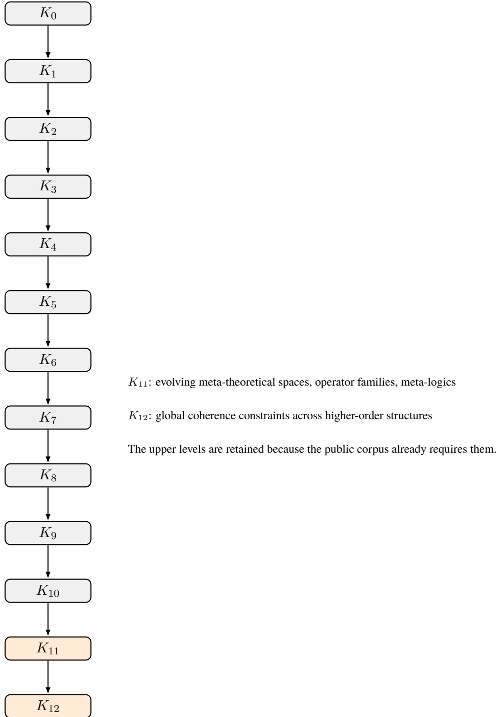
Figure 9: vertical hierarchy of continua from K_0 to K_{12} .
