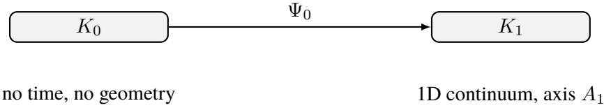
Figure 8: Schematic of the transition \Psi_{0 \rightarrow 1} from the substrate K_0 to the first continuum K_1 .
