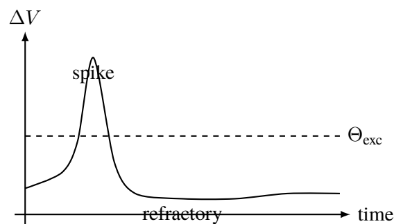
Figure 52: Proto-spike dynamics as a minimal excitatory cycle.
