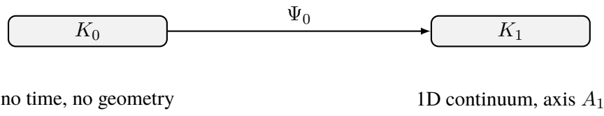
Figure 37: Schematic of the transition \Psi_{0 \rightarrow 1} from the substrate K_0 to the first continuum K_1 .
