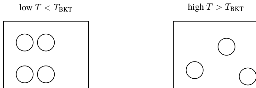
Figure 43: BKT-type transition as an example of threshold-governed emergence of a new topological axis.
