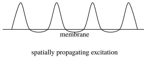
Figure 50: Propagation of membrane potential \Delta V along a boundary.
