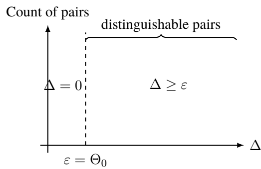
Figure 36: Structural difference and minimal threshold \Theta_0 at level K_0 .
