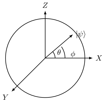
Figure 44: Illustrative Bloch sphere diagram for quantum two-level systems.
