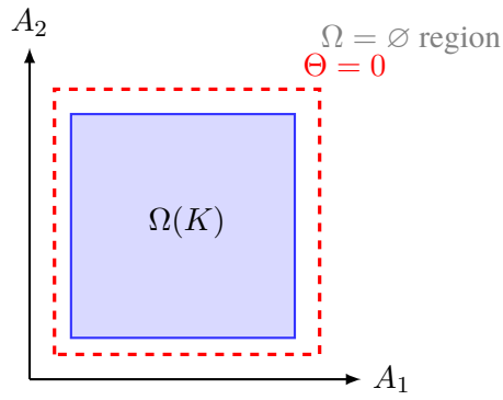
Figure 34: Axes and threshold surfaces in the extended state space of a continuum.
