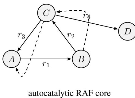
Figure 45: RAF network as a chemical continuum at level K_3 .
