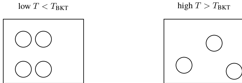
Abbildung 14: BKT-type transition as an example of threshold-governed emergence of a new topological axis.
