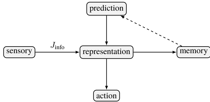
Abbildung 31: Flows between representations, models and data in K_9 .
