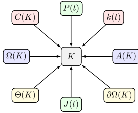
Abbildung 4: Schematic structure of a continuum K = (\Omega, A, P, J, \Theta, \partial\Omega, C, k) .
