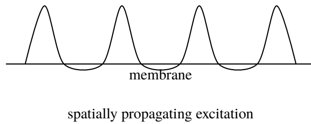
Abbildung 21: Propagation of membrane potential \Delta V along a boundary.
