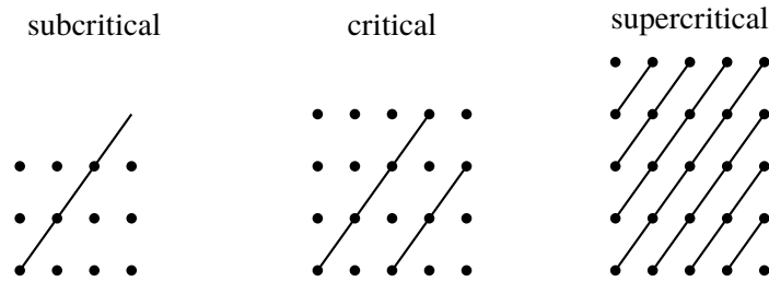
Abbildung 13: Percolation-type transition at level K_2 .
