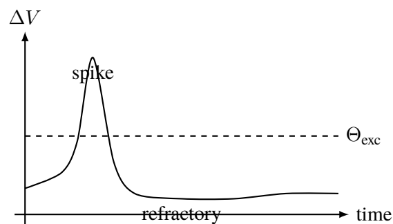
Abbildung 23: Proto-spike dynamics as a minimal excitatory cycle.
