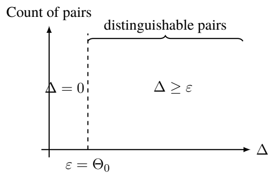
Abbildung 7: Structural difference and minimal threshold \Theta_0 at level K_0 .
