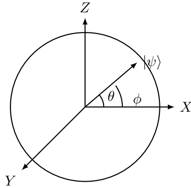
Abbildung 15: Illustrative Bloch sphere diagram for quantum two-level systems.
