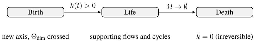
Abbildung 2: Minimal life-cycle schematic for the bounded collapse grammar. The point of the figure is not to offer a domain-specific simulation but to show the exact interpretive burden of the formal rules: positive continuumness keeps the object live; admissible-state collapse kills it; any later continuation must be classified under rebirth rather than persistence.
