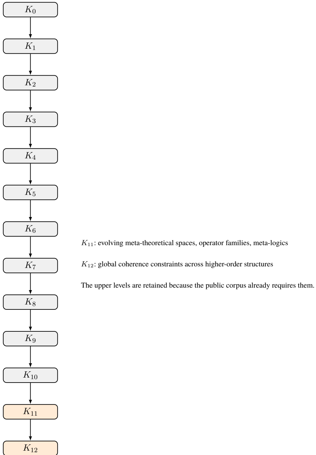
Abbildung 3: Extended vertical hierarchy through K_{12} . The added upper levels are justified by the need to represent evolving meta-theoretical spaces and their global coherence conditions rather than by decorative level inflation.
