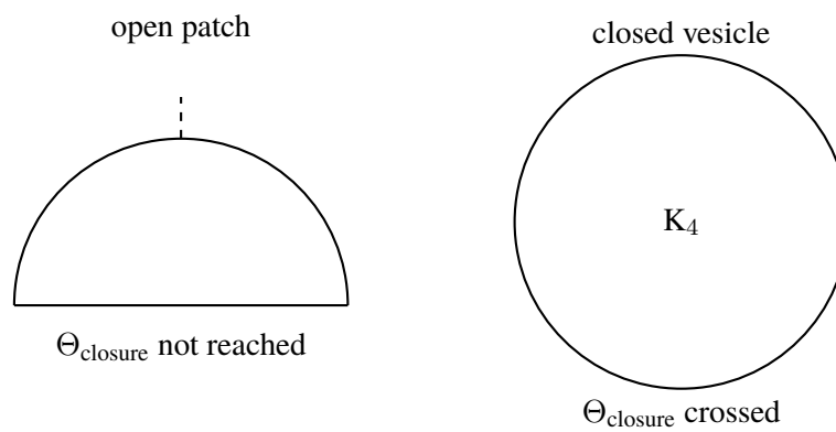
Abbildung 18: Membrane closure and emergence of a protocellular boundary at level K_4 .
