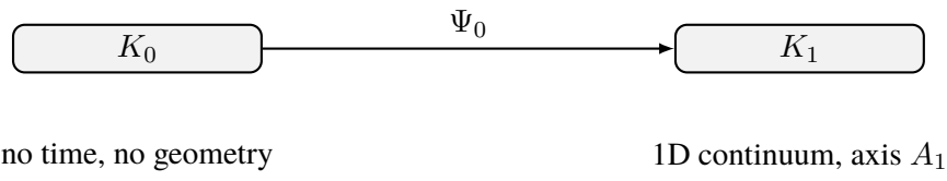
Abbildung 8: Schematic of the transition \Psi_{0 \rightarrow 1} from the substrate K_0 to the first continuum K_1 .
