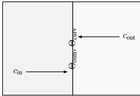
Figure 19: Osmotic gradients, membrane tension and structural thresholds in protocells.
