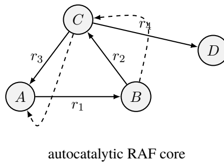
Figure 16: RAF network as a chemical continuum at level K_3 .
