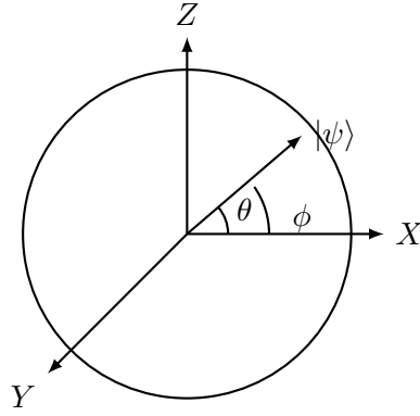
Figure 15: Illustrative Bloch sphere diagram for quantum two-level systems.
