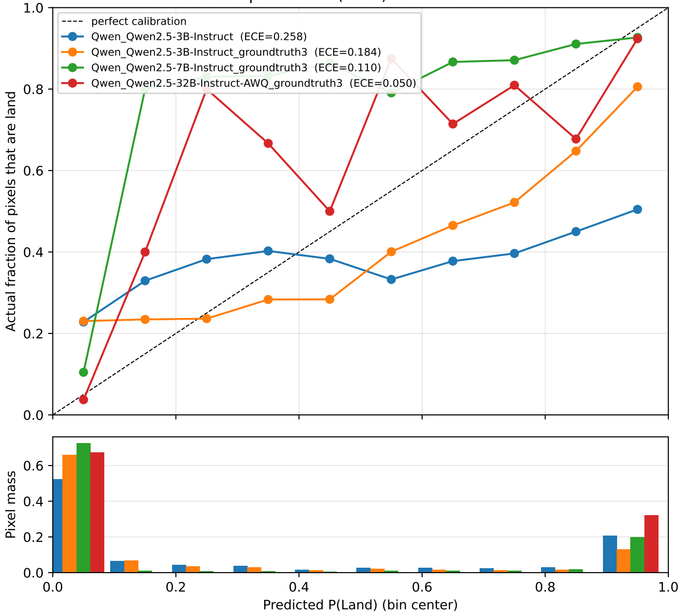
Calibration: predicted P(Land) vs. observed land rate
