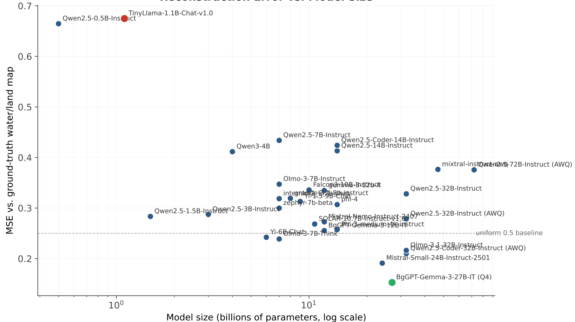
Reconstruction Error vs. Model Size
