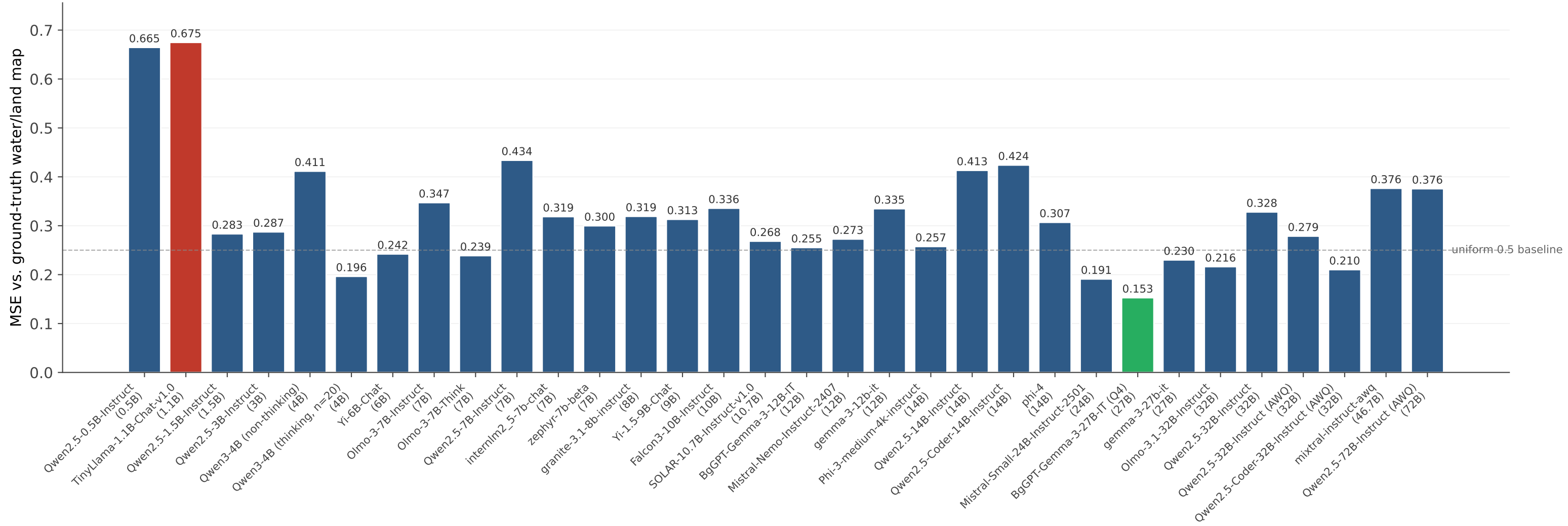
Reconstruction Error by Model (sorted by parameter count)
