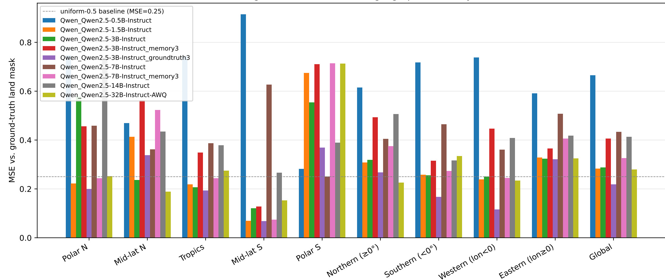
Per-region MSE (lower = better geographic accuracy)
