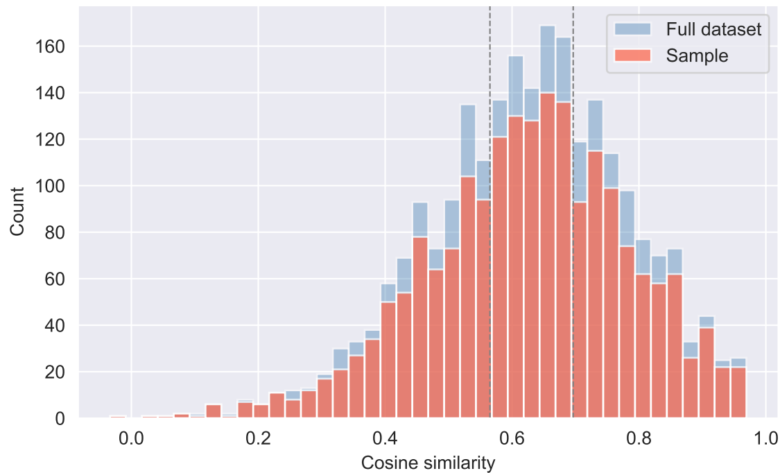
Similarity distribution — full vs sample
