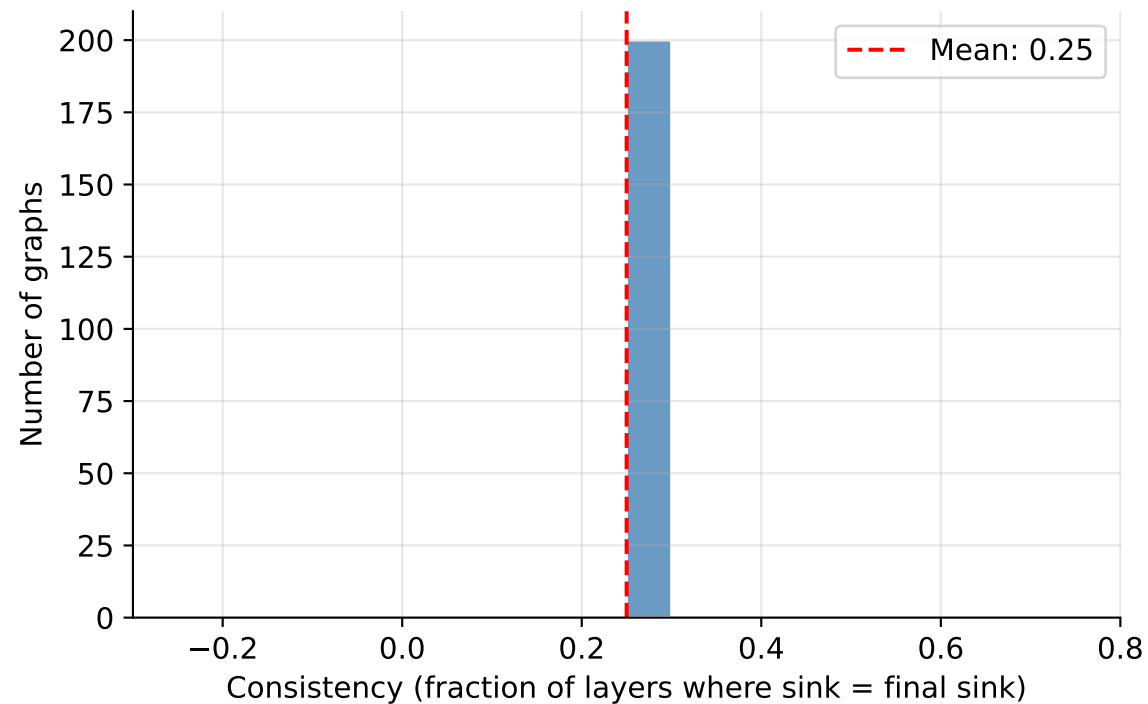
PascalVOC (no VNode, ~479 nodes)
