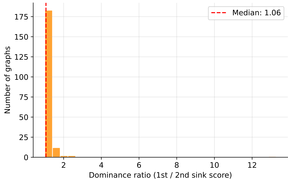
ZINC (no VNode, ~23 nodes)
