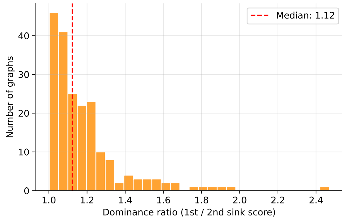
PascalVOC (no VNode, ~479 nodes)
