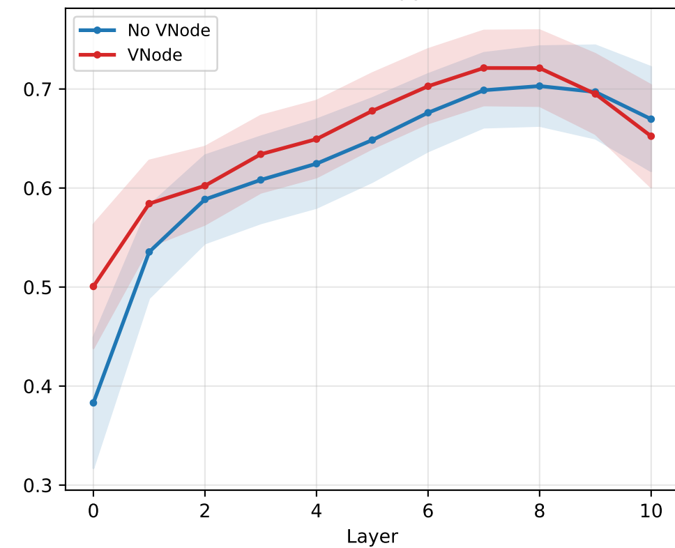
Norm Ratio
