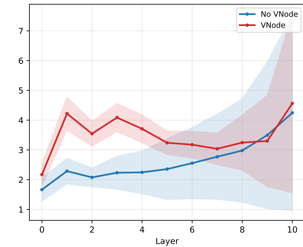
Norm Ratio
