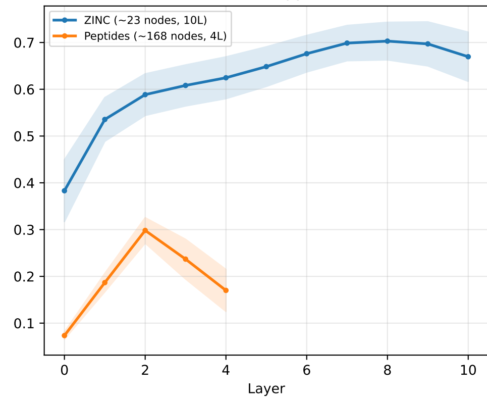
Norm Ratio
