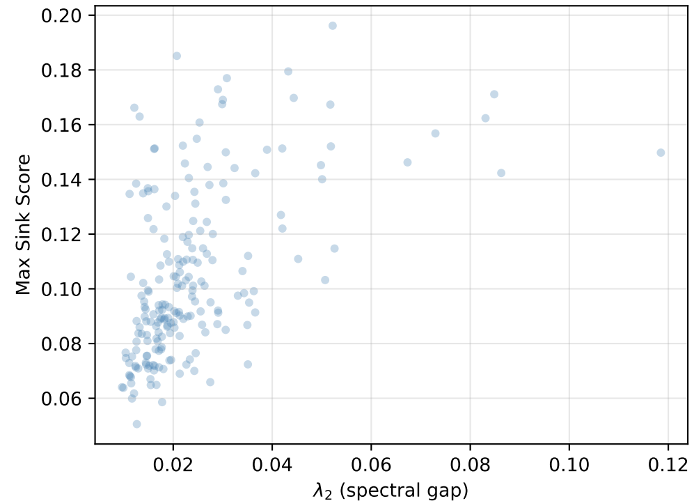
ZINC (no VNode, ~23 nodes) \lambda_2 vs max sink score ( r=0.554 , p=1.7e-17 )
