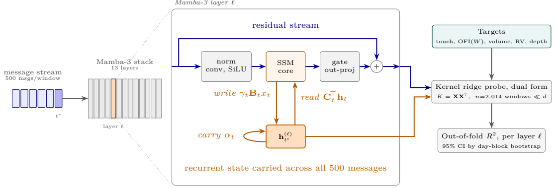
Figure 5.1: Probing loci in a message-only Mamba-3 model. From each layer we extract the per-token residual stream and the recurrent state \mathbf{h}_t^{(\ell)} , which accumulates across all messages of the window. Both are read out by the same kernel ridge probe.
