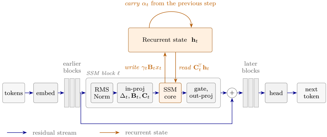
Figure 2.3: A state-space model with a focus on a single block inside the stack. The block normalises the stream, projects the token into \Delta_t , \mathbf{B}_t and \mathbf{C}_t , passes it through the recurrence, gates it and adds the result back. The recurrent state is carried from the past, attenuated by \alpha_t , written into through \mathbf{B}_t and read from through \mathbf{C}_t . Its size is fixed, so the cost per message does not grow with the length of the rollout.
