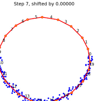
(e) \alpha = 1.00
