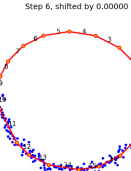
(c) \alpha = 0.05
