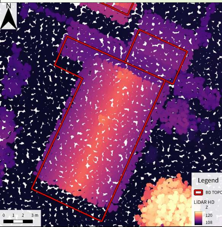
4. 3D roof model
