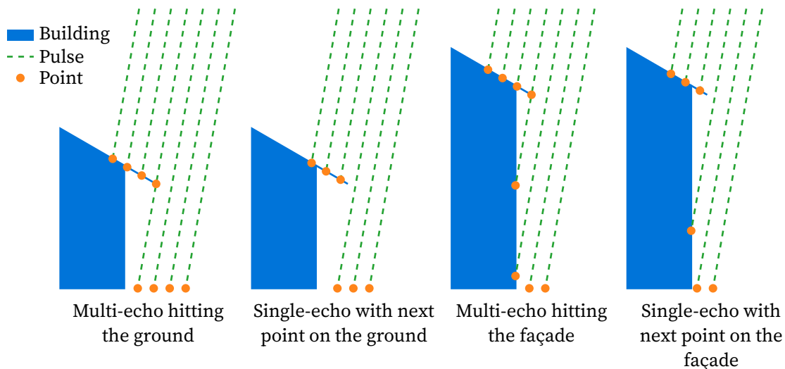
Figure 8: Illustration in profile view of the lack or sparsity of points on the façades.
