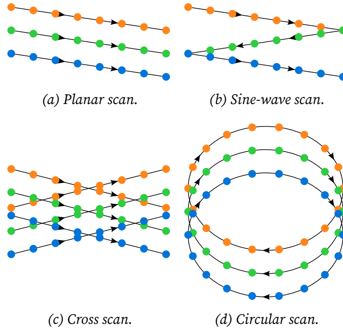
Figure 3: Illustration of different types of ALS sensors, with multiple consecutive scan lines in orange, green and blue (the scanning vehicle is moving towards the bottom of the figures), inspired from (Wu et al., 2026).
