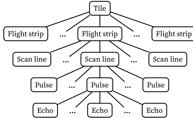
Figure 4: Illustration of the topological structure of a tile of an ALS point cloud.
