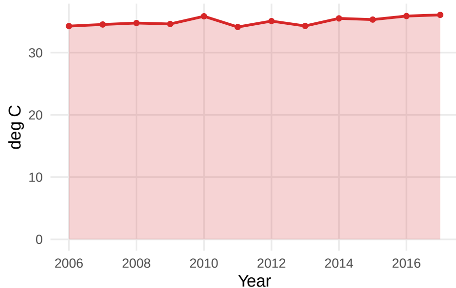
(c) Land surface temperature
