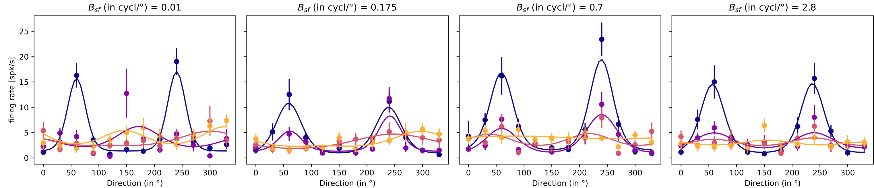
neuron 1
