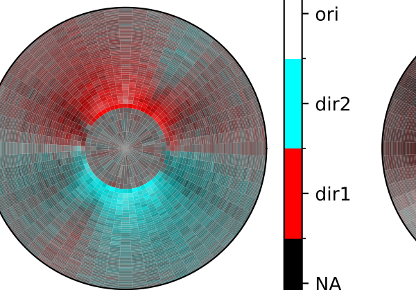
neuron 2
