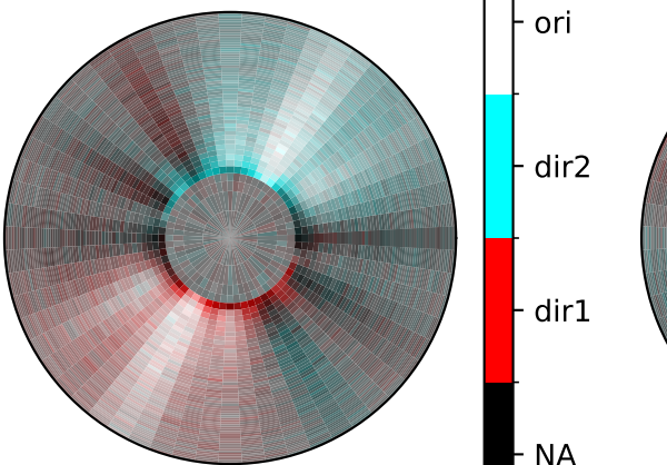
neuron 1
