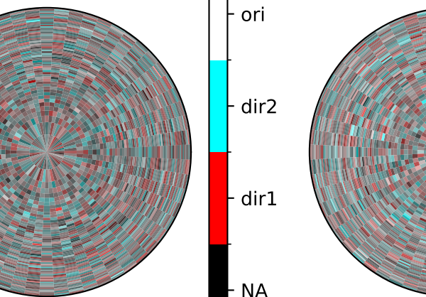
neuron 8
