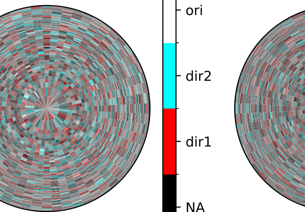
neuron 7
