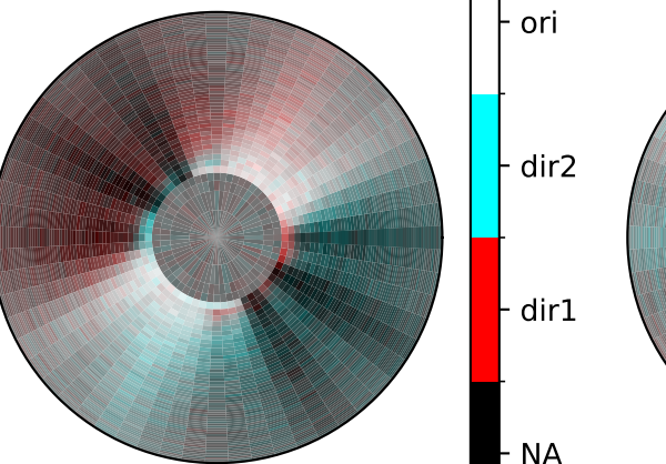
neuron 3
