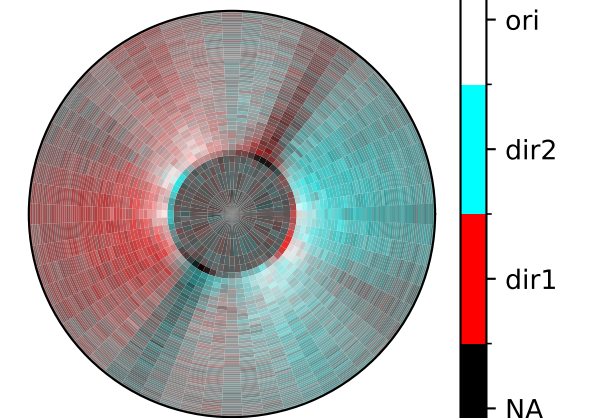
neuron 0
