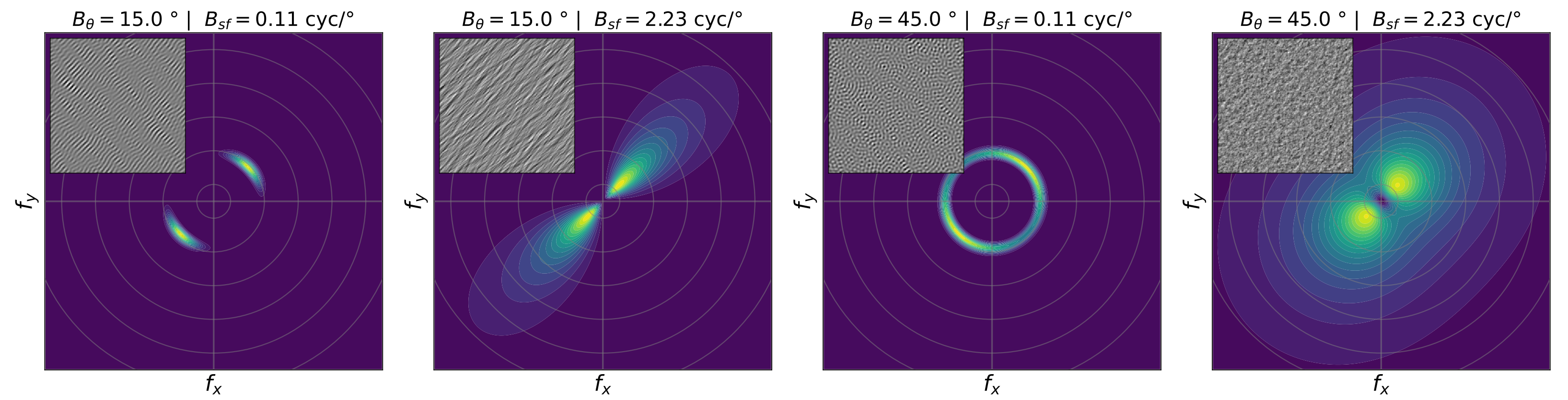
Figure 2: Fourier space representation of MotionClouds stimuli. The image is generated by the inverse fourier transform of the envelop after the application of a random phase.
