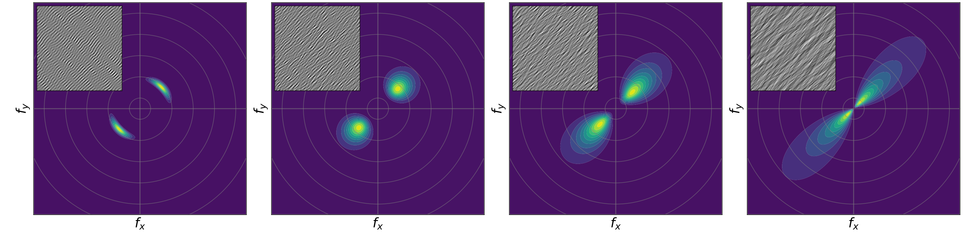
Figure 1: Fourier space representation of MotionClouds stimuli. The image is generated by the inverse fourier transform after the application of a random phase.
