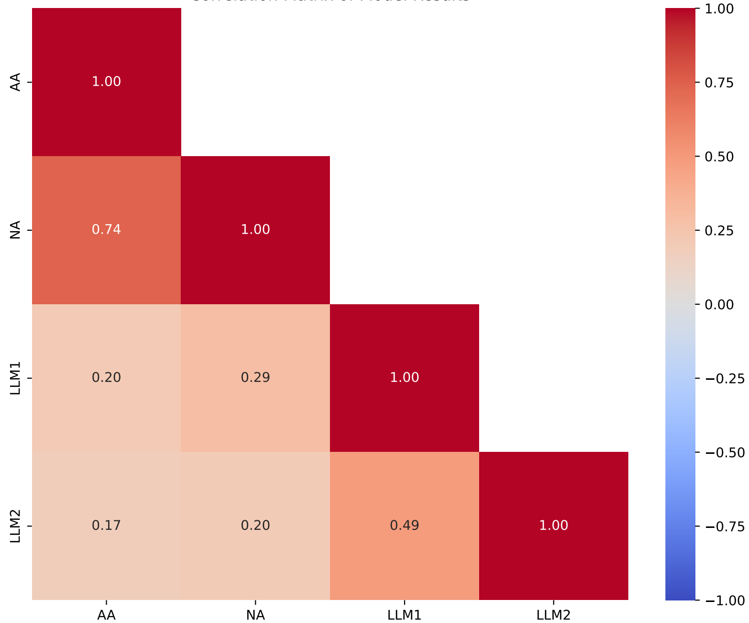
Correlation Matrix of Model Results
