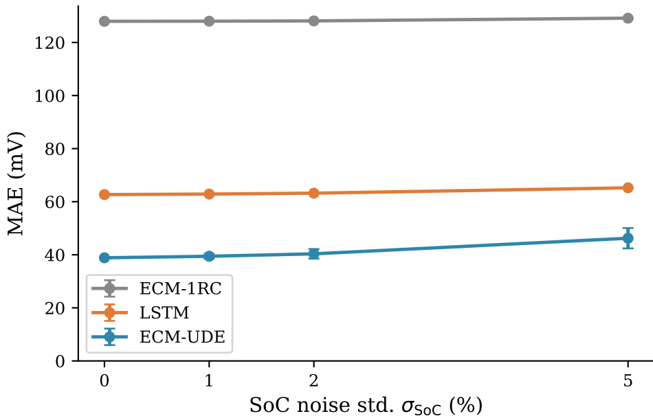
Sensitivity to inference-time SoC uncertainty Gaussian noise added to the SoC input channel
