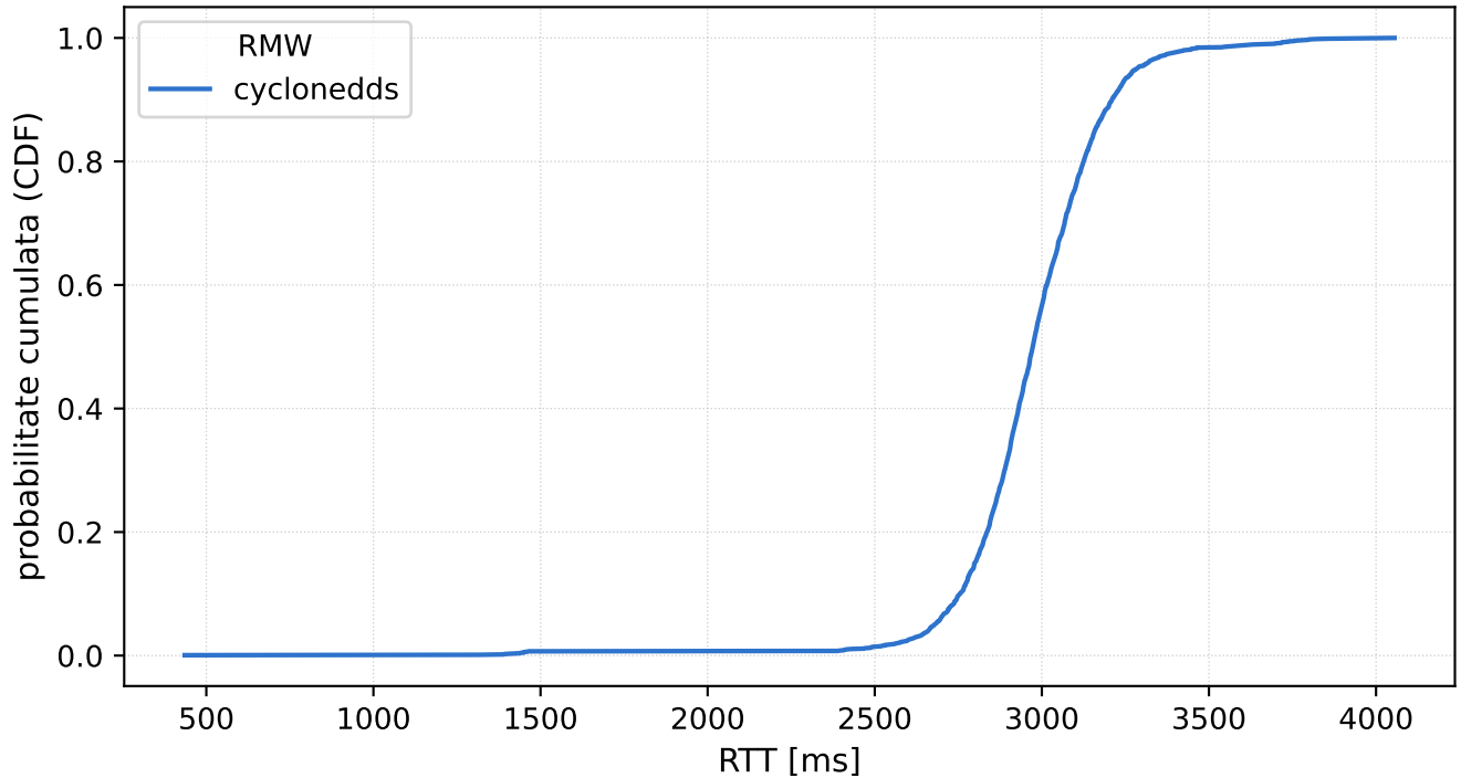
Distributia RTT -- conditia 'lat200_l15'
