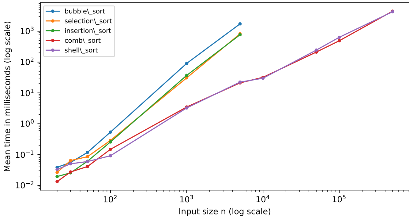
Small and quadratic-family algorithms on random integers
