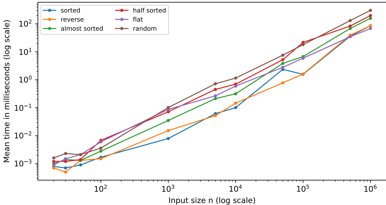
Timsort sensitivity to input structure on integers
