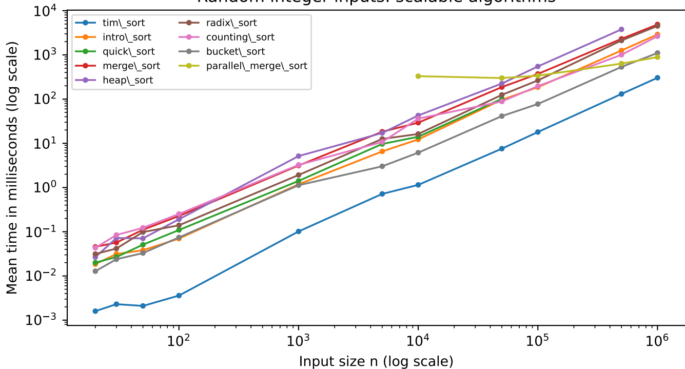
Random integer inputs: scalable algorithms
