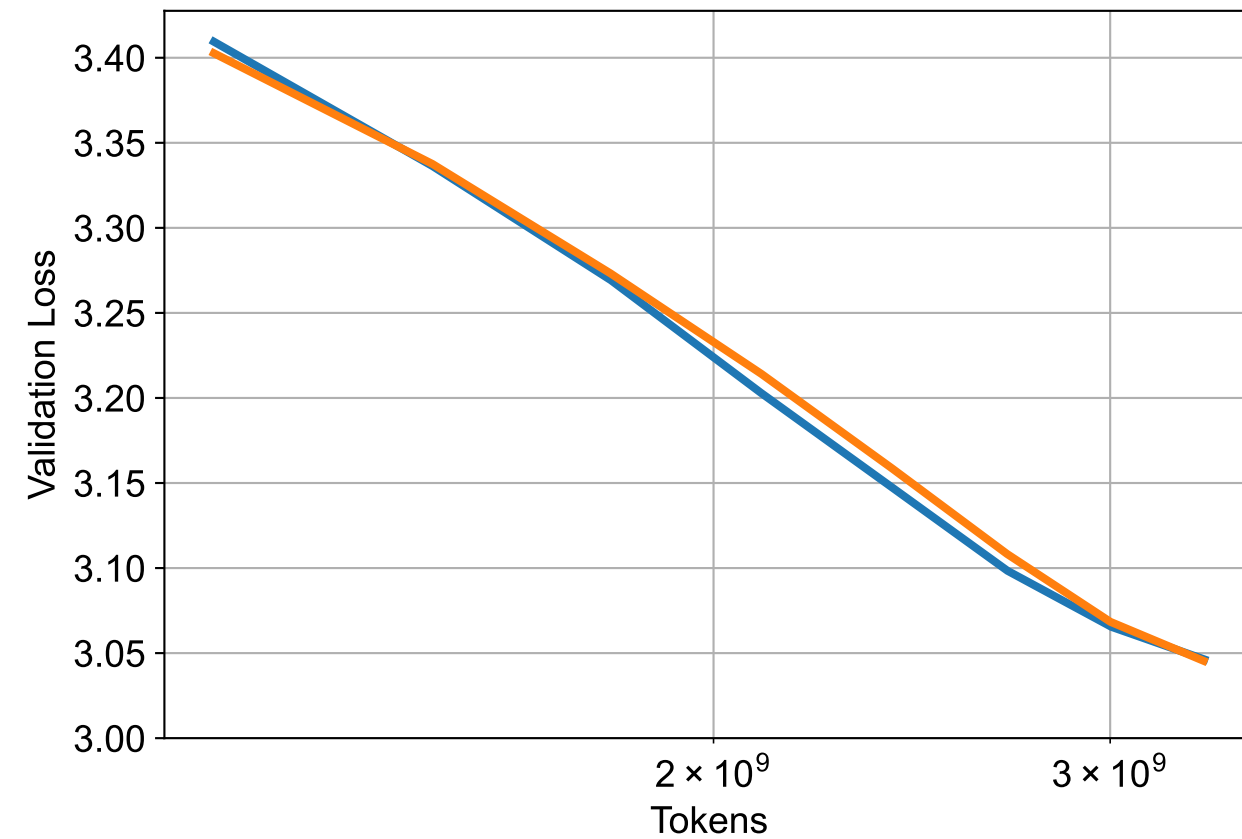
Batch Size: 512
