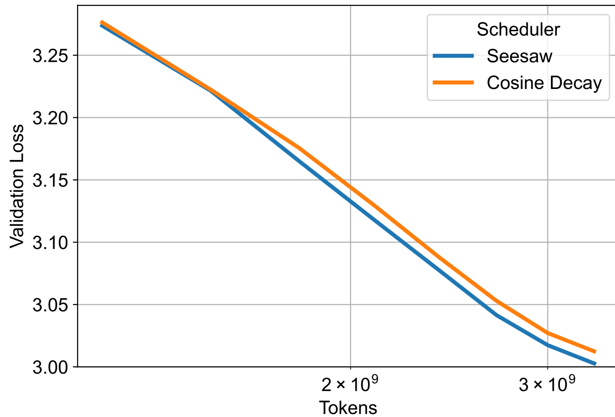
Batch Size: 128
