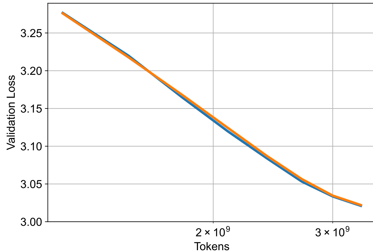
Batch Size: 256
