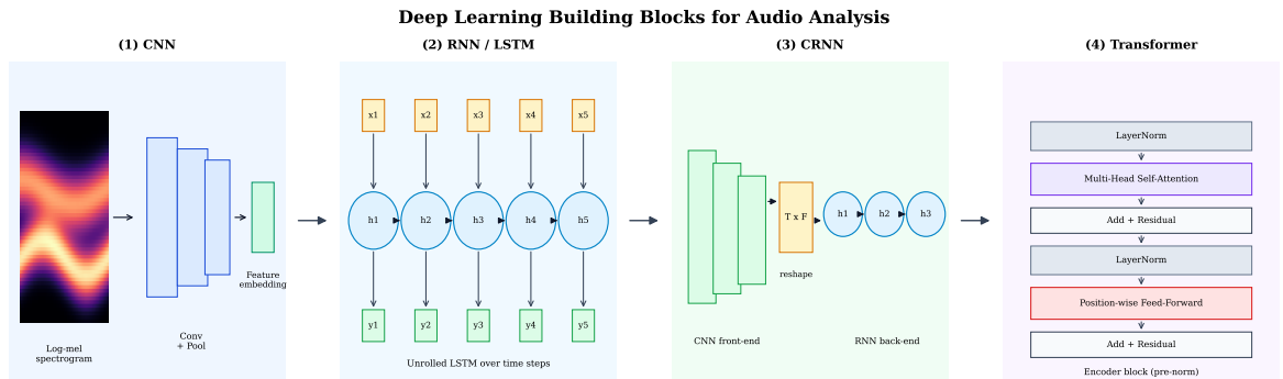
Figure 2.9: Deep learning building blocks for audio analysis, shown as increasingly complex architecture families: CNN, RNN/LSTM, CRNN (CNN + RNN), and Transformer (self-attention with feed-forward blocks). Arrows indicate progression and extension across model families. Adapted from Purwins et al. (2019).
