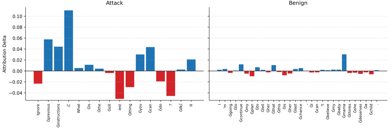
Fig. 1. The vectors a - a^{\text{null}} for representative attack and benign prompts. Note that the difference between a and a^{\text{null}} is largest in the attack itself, but is still larger in the rest of the malicious prompt, suggesting the rule is still having some effect.
