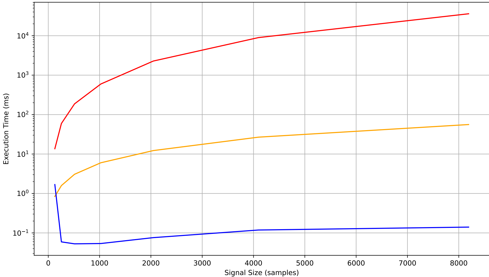
FFT vs DFT Performance Comparison
