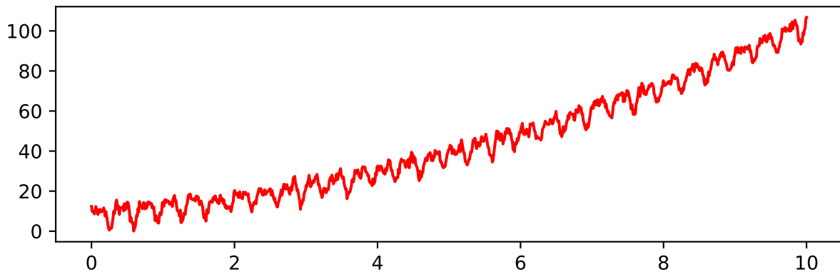
Exponential smoothing simplu
