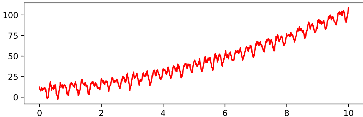
Triple exp (alpha=0.4, beta=0.3, gamma=0.2)
