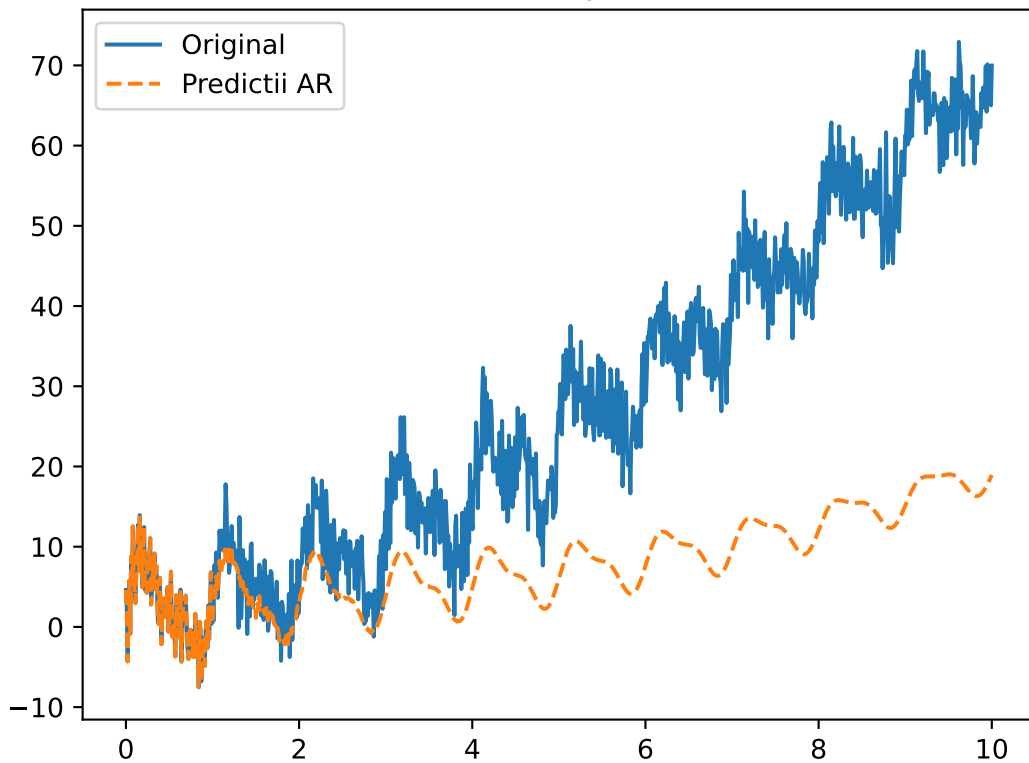
Model AR (p=100)
