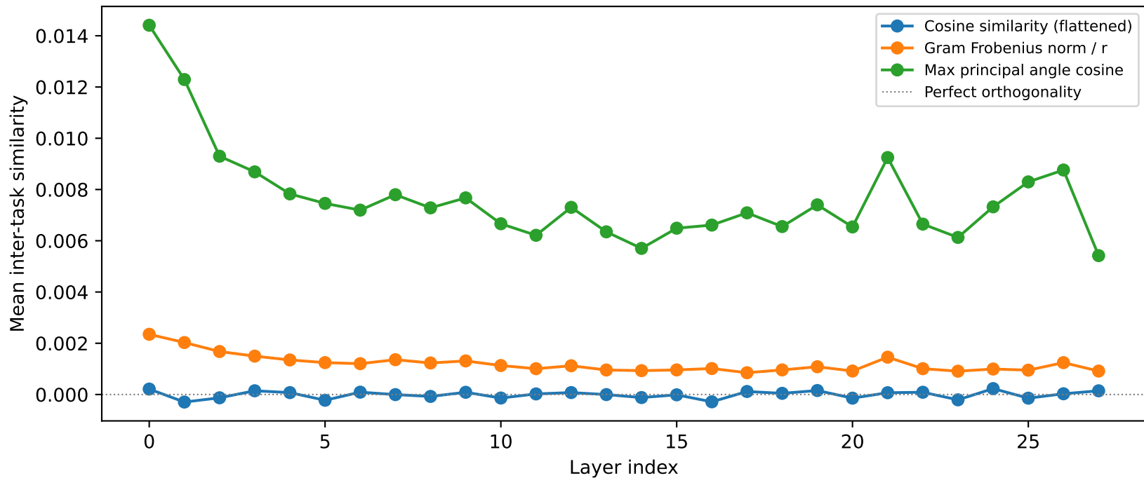
Layer-wise orthogonality (A matrices) — olora
