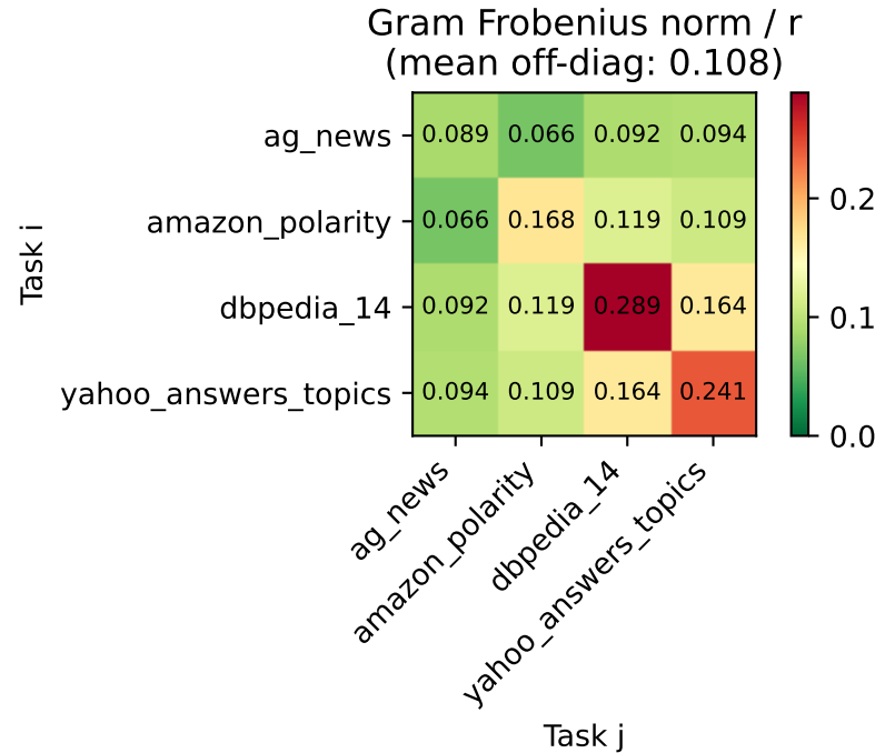
olora — task-pair similarity (B matrices)
