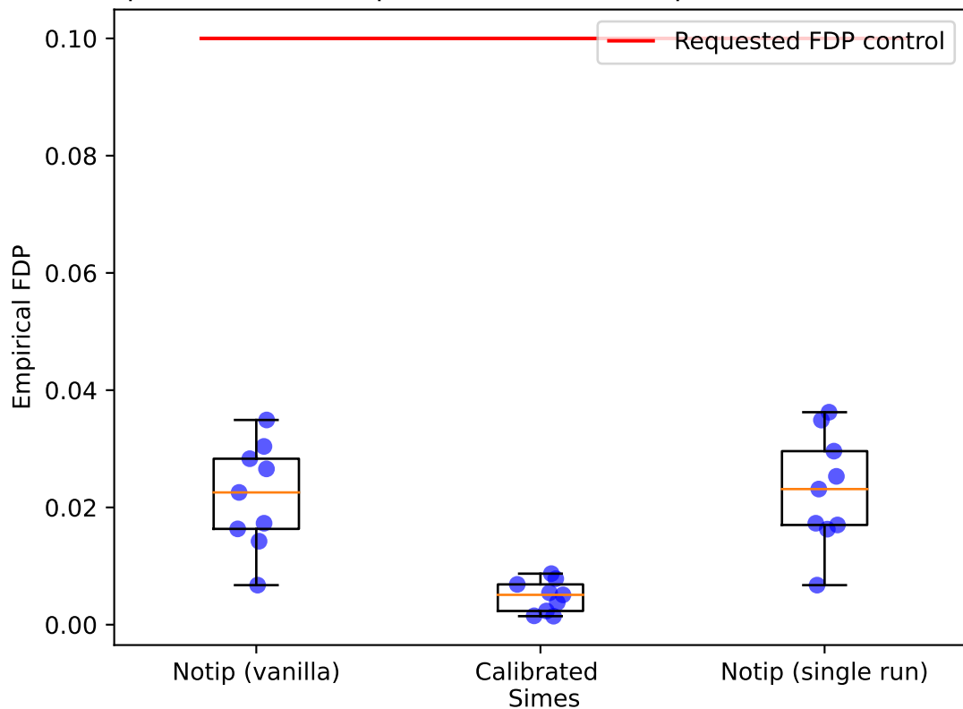
Empirical FDP for requested FDP control q = 0.1 at level \alpha=0.05
