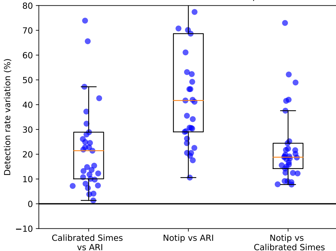
Detection rate variation for \alpha = 0.05, FDP \leq 0.1
