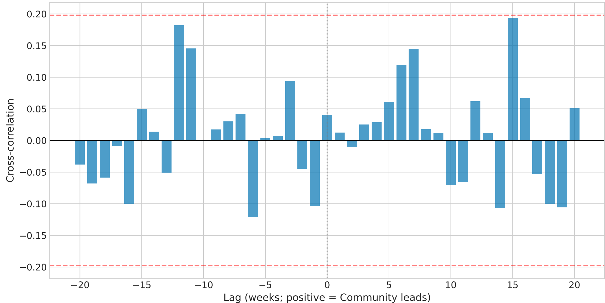
Cross-Correlation: Zeiger vs. Community Siege Score
